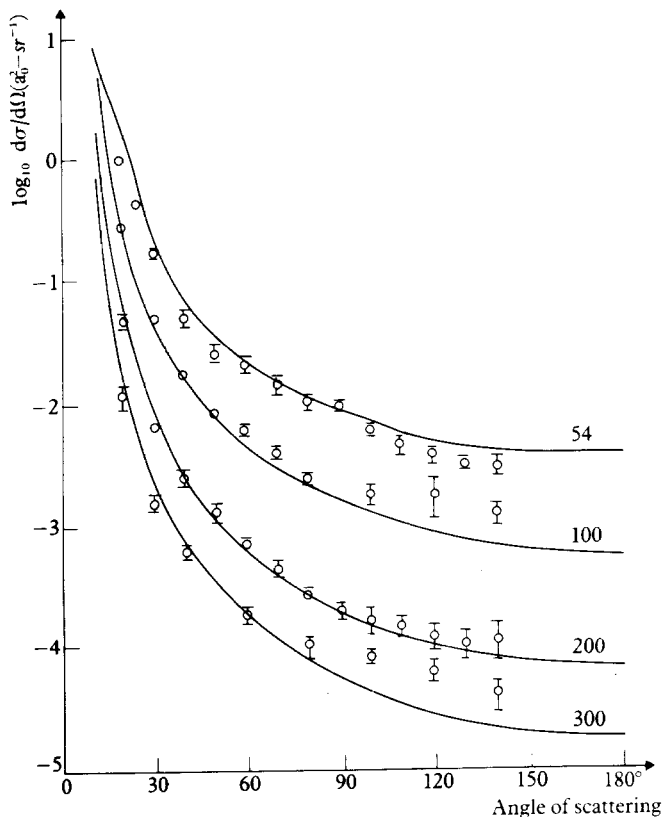
12.5 The cross-section for excitation of the (2s + 2p) levels of hydrogen by electron impact at 54, 100, 200 and 300 eV. The solid line is the result of a three-state close-coupling approximation.
